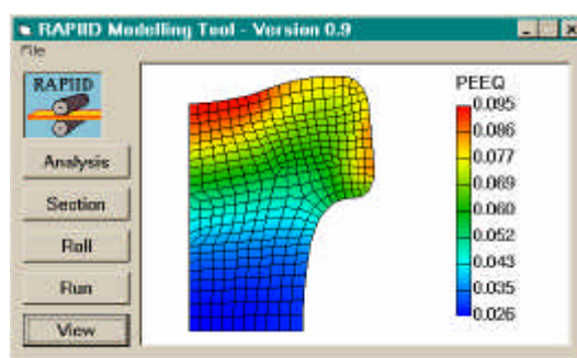
Rapid Prototyping RAPIID 2.5D FEM Code
